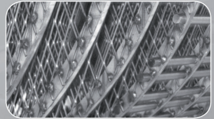
An EMbaffle® close up
