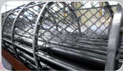
An example of an 18 metre, Compact EMbaffle® Gas/Gas heat exchanger under fabrication
